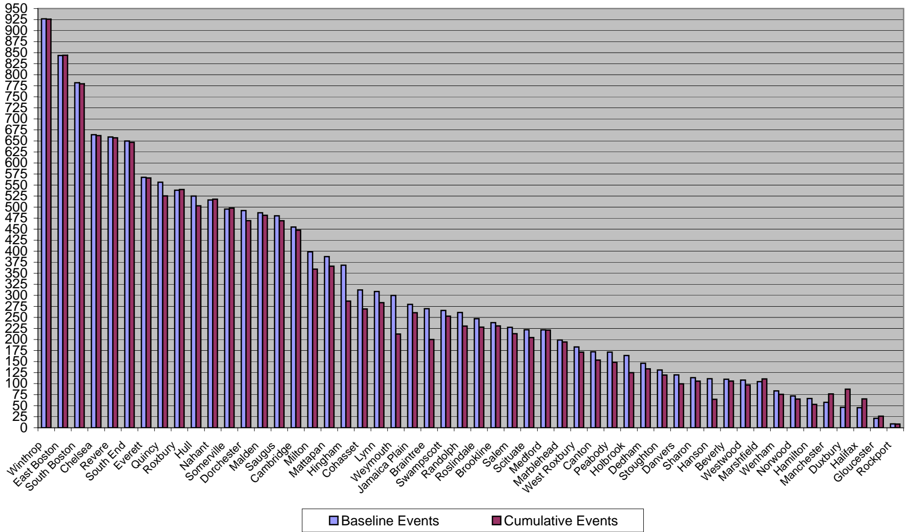
Graph 1 - Phase 1 BLANS Alternatives Community Average Baseline and Cumulative Average Daily Events Above 50 SEL (Level Approximates Ambient Noise in Quiet Suburb)
