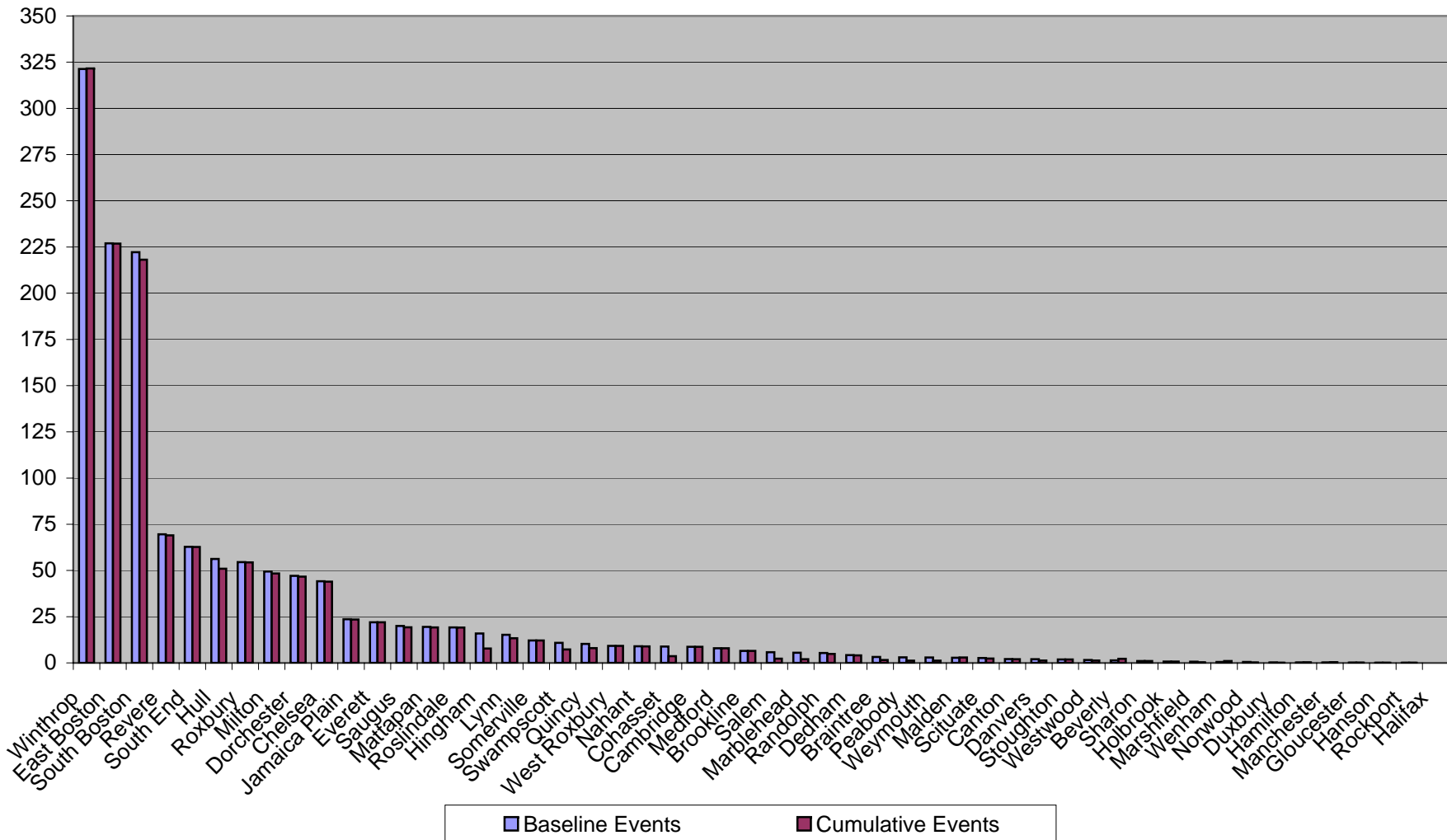
Graph 5 - Phase 1 BLANS Alternatives Baseline and Cumulative Average Daily Events Above 75 SEL (Level Approximates Noise Level in a Busy Restaurant or Normal Conversation at 3 Feet)
